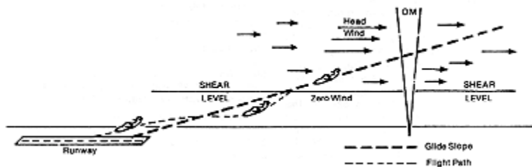
Figure 6 Moderate shear-at altitude where over-corrections results in long landing or overshoot.
